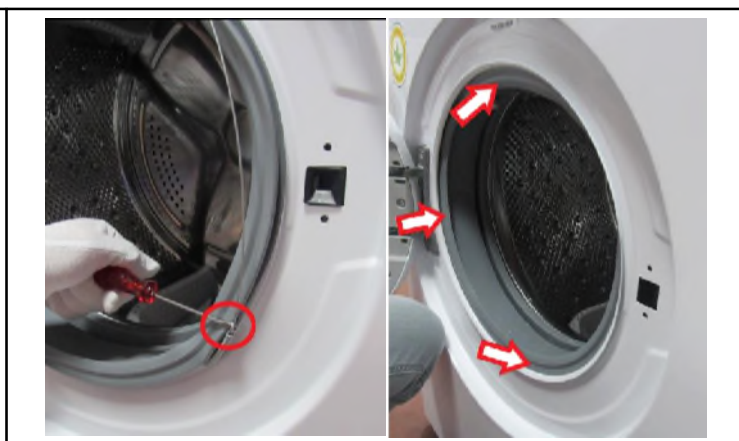
2.9. Remove the wire by using small screwdriver and push the seal to the inside
