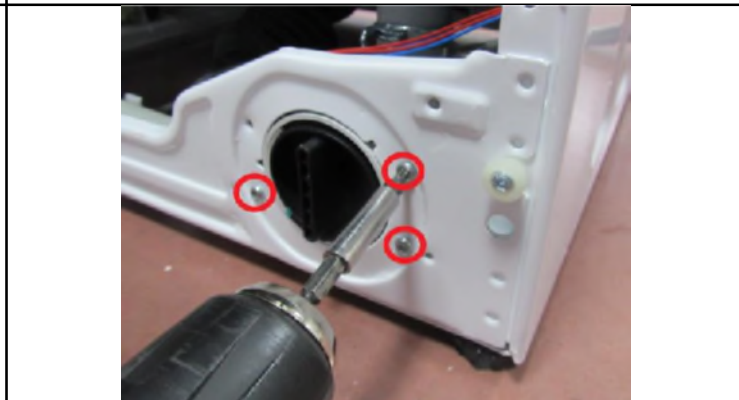
2.11. Remove screws holding drain pump
