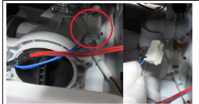
2.12. Remove the drain pump connector
