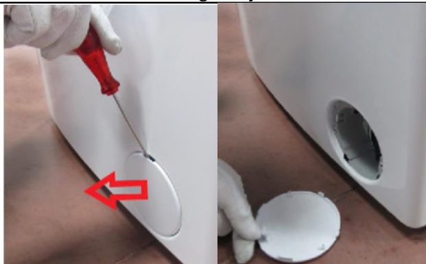
2.7. Remove the screw and plastic part located under the pump cover
