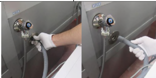
1.2. Turn off the tap and disconnect the hose from the valve
