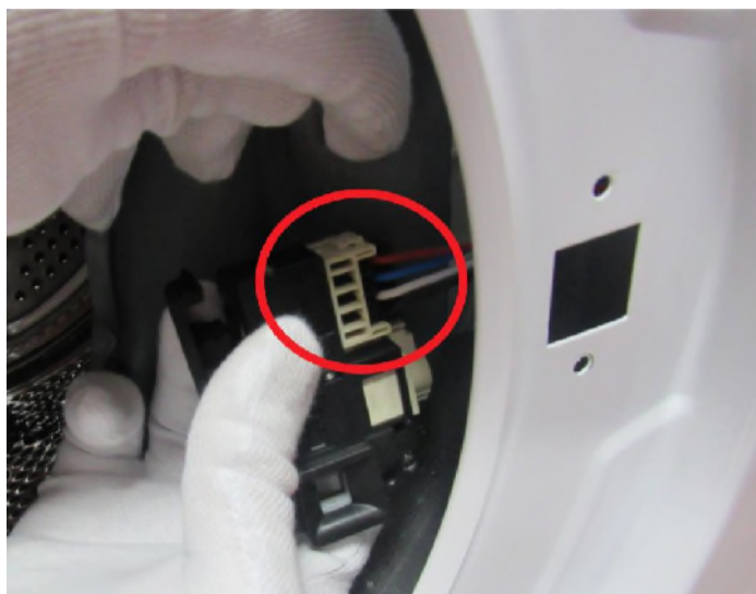
4.1 Unplug the connector and remove the door lock. Connect the new door lock to connector.
