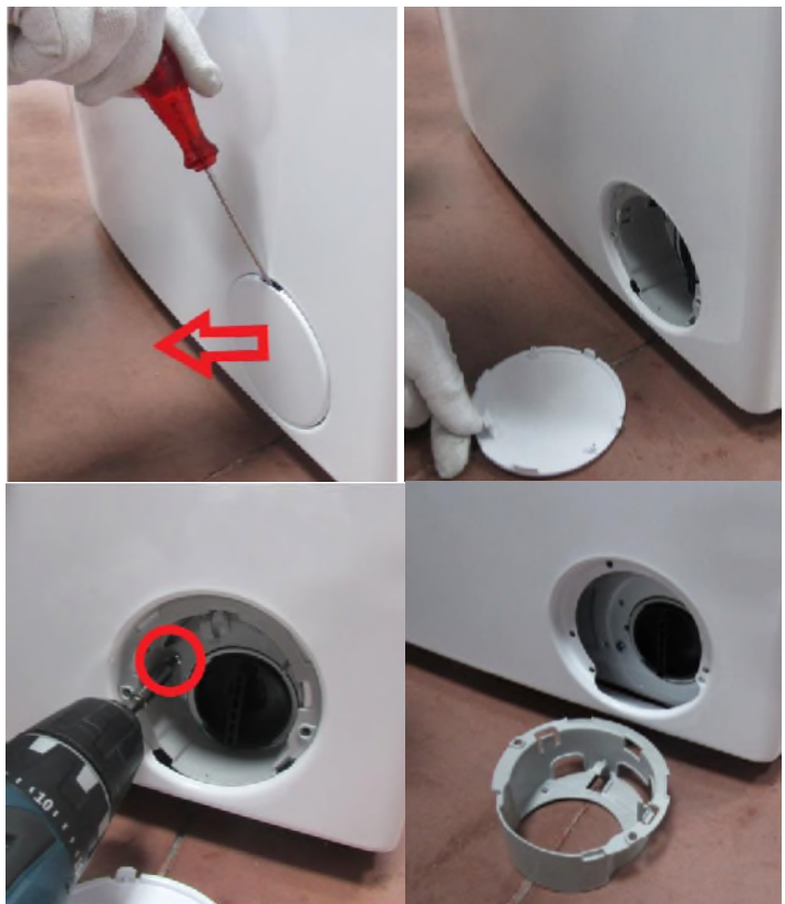
3.9 Remove the screw and plastic part located under the pump cover
