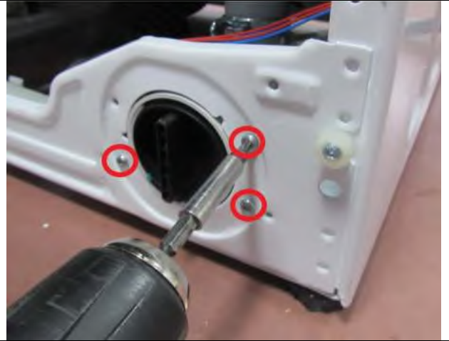
3.4. Tighten the screws holding drain pump
