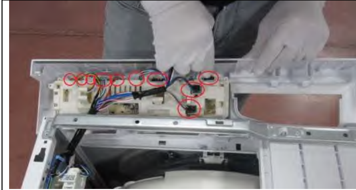
3.3. Connect the all sockets on the card according to the wiring diagram.
