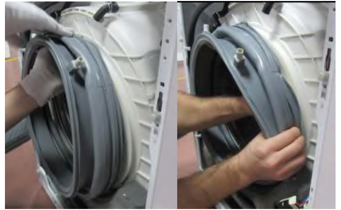
3.1.2. Fit the tub bellow seal to the front tub
