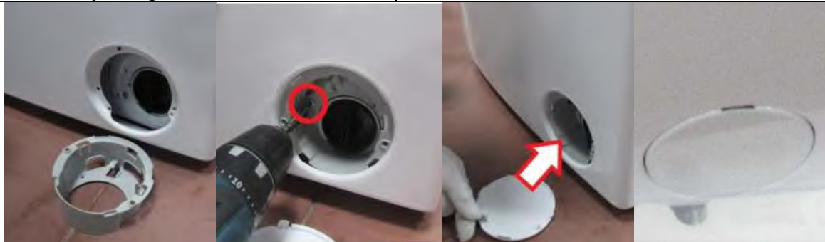
3.7. Tighten the screw and plastic part located under the pump cover
