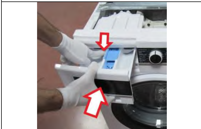
3.12. While pressing siphon cover keep pushing drawer to fit it.
