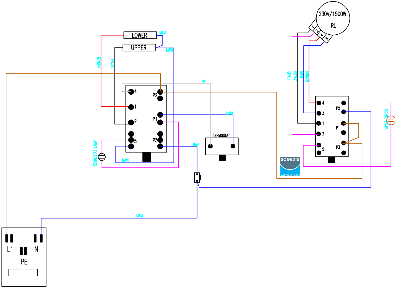
TERMINAL BOX
