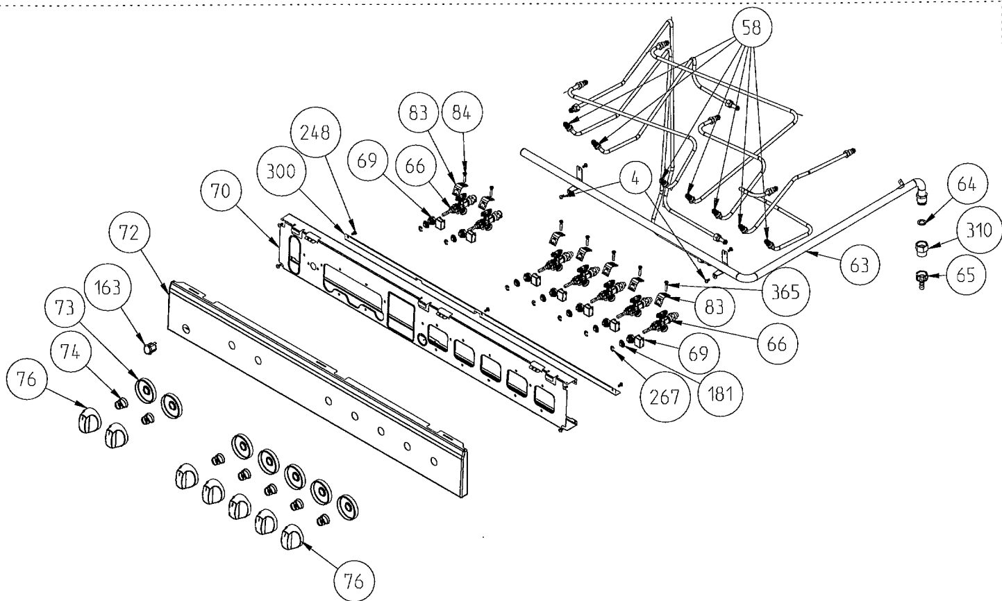
5 GAS COOKTOP WITHOUT OVEN THERMOSTAT (SEPERATE KNO B CONTROL)
