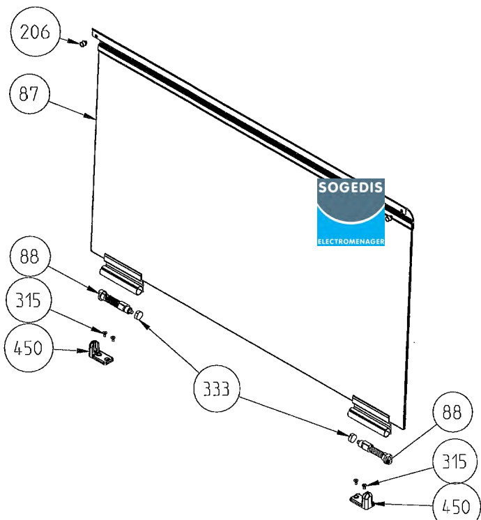
GLASS LID COVER ASSEMBLY WITH PROFILE
