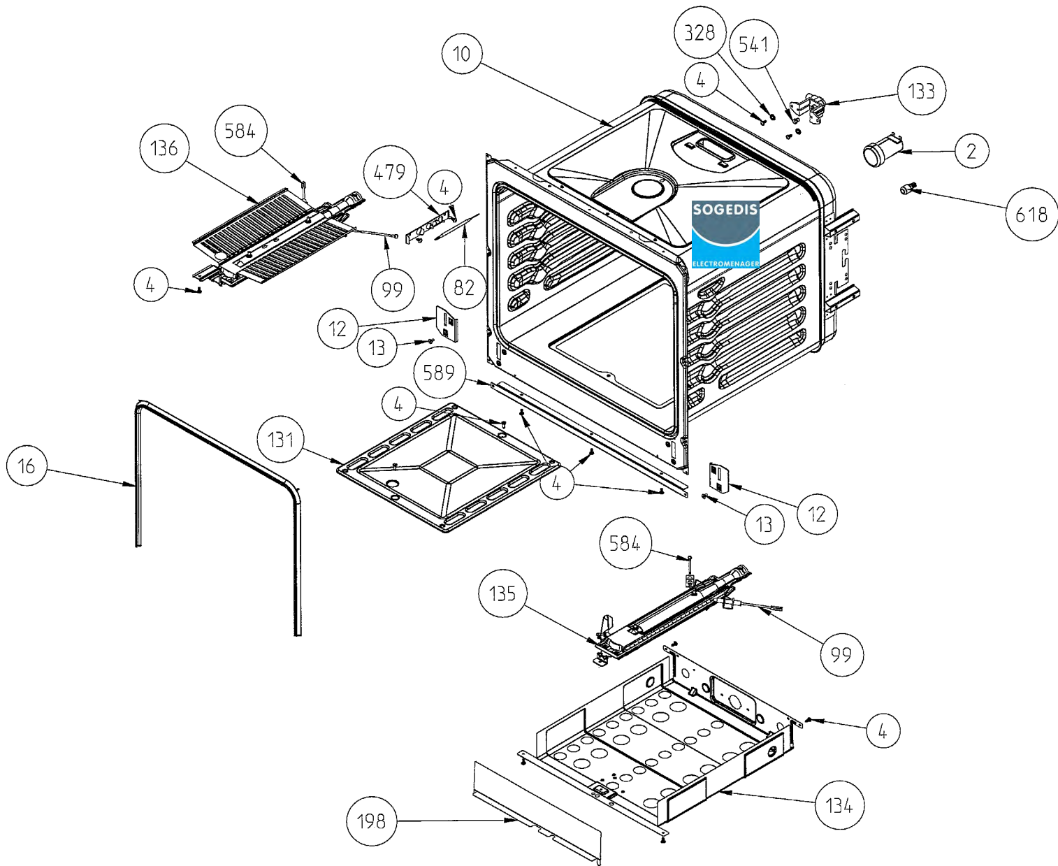
GAS OVEN GAS GRILL CAVITY ASSEMBLY
