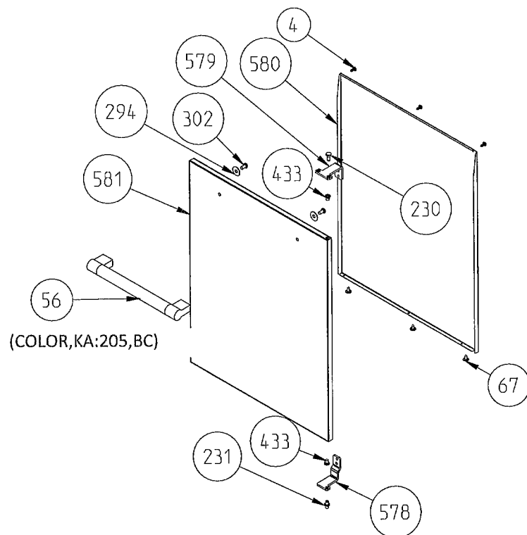
BOTTLE COMPARTMENT DOOR
