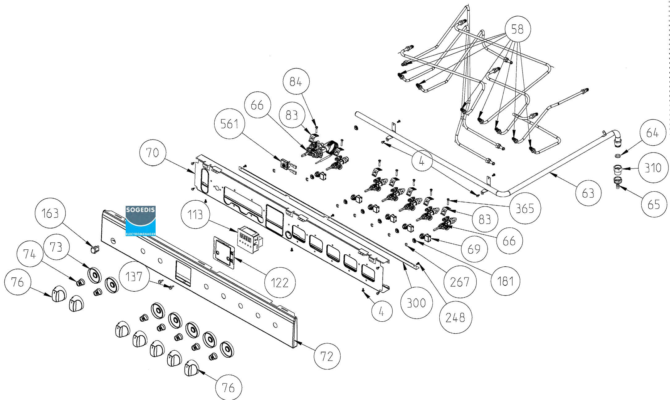
5 GAS COOKTOP WITH OVEN THERMOSTAT (SEPERATE KNO B CONTROL ,DIGITAL TIMER)
