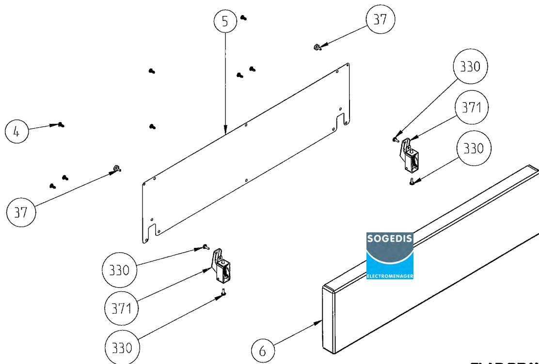
FLAP DRAWER ASSEMBLY
