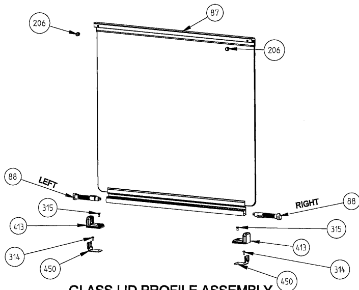
GLASS LID PROFILE ASSEMBLY (OPTIONAL)
