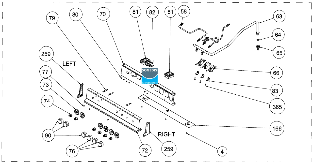
3G-1E CONTROL PANEL ASSEMBLY
