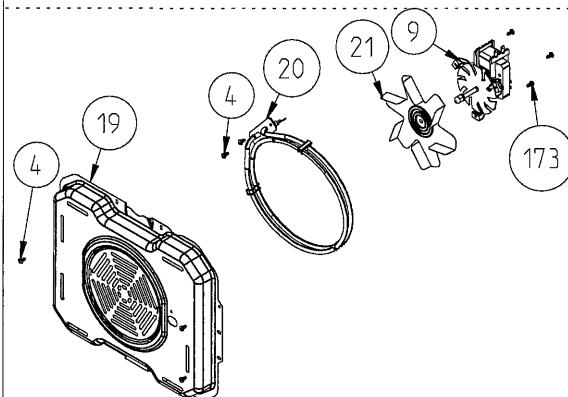
RING HEATING ELEMENT WITH FAN (OPTIONAL)
