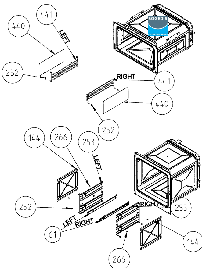
WIRE SHELF CAVITY ASSEMBLY WITH / WITHOUT CATALYTIC PANEL OPTIONAL :TELESCOPIC RAIL (R / L)
