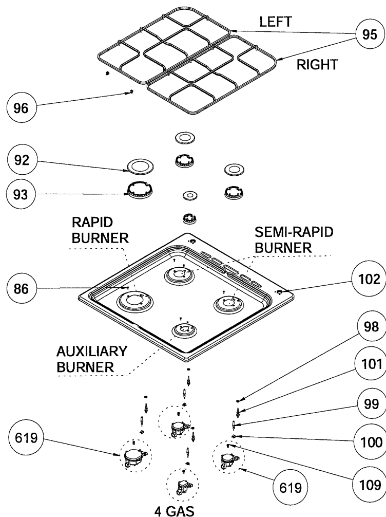
EXPLODED VIEW - COOKTOP ASSEMBLY
