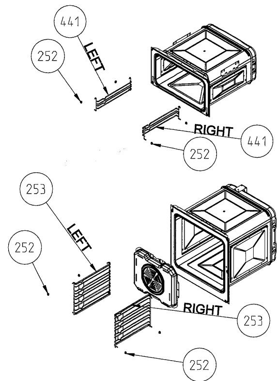
CAVITY ASSEMBLY WITH WIRE SHELF (OPTIONAL)
