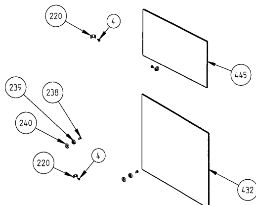
THIRD GLASS (REMOVABLE) OVEN DOOR VERSION (OPTIONAL)
