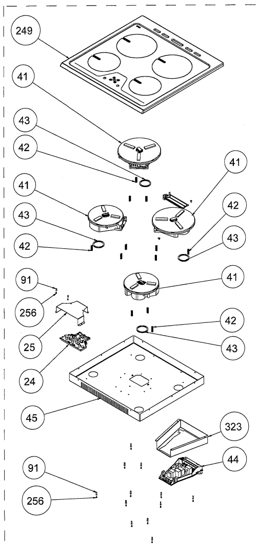
TOUCH CONTROL COOKTOP ASSEMBLY
