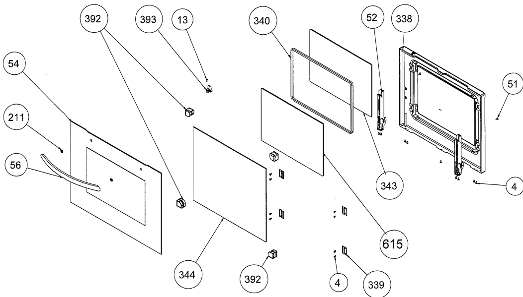
OVEN DOOR ASSEMBLY (OUTER & INNER) (POSITION NO 378)
