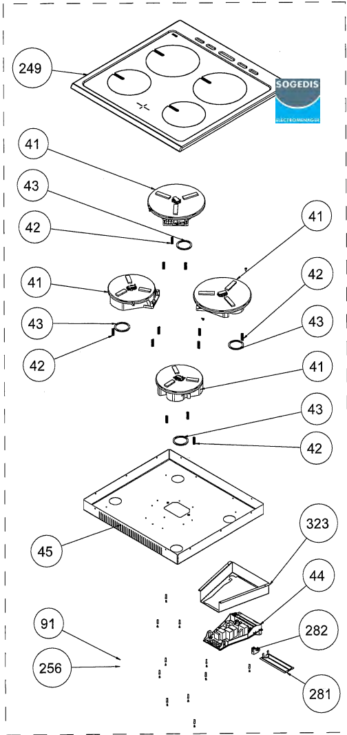
KNOB CONTROL COOKTOP ASSEMBLY
