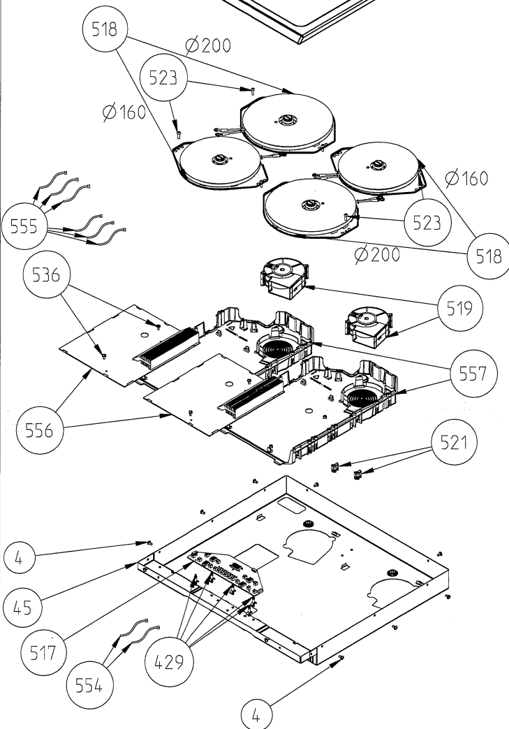
TOUCH CONTROL SLIDER COOKTOP ASSEMBLY
