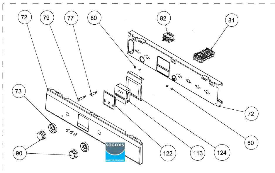
TOUCH CONTROL PANEL ASSEMBLY
