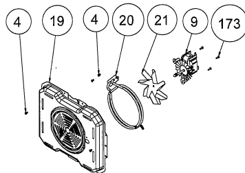
RING HEATING ELEMENT WITH FAN ( OPTIONAL )
