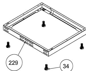
EXTRA BOTTOM SUPPORT (WITH LOUVRES)
