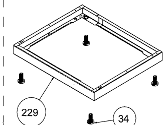
ADDITIONAL BOTTOM SUPPORT
